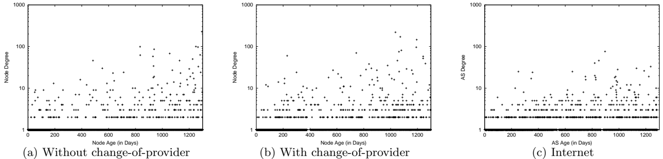
Figure 7: Age-degree correlation
