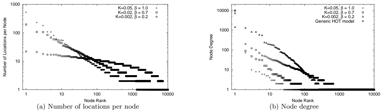
Figure 2: The modified HOT model ( \alpha=5 and n=10,000 )
