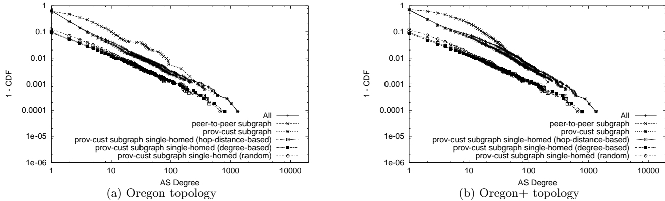
Figure 1: Node degree distributions of AS (sub)graphs.
